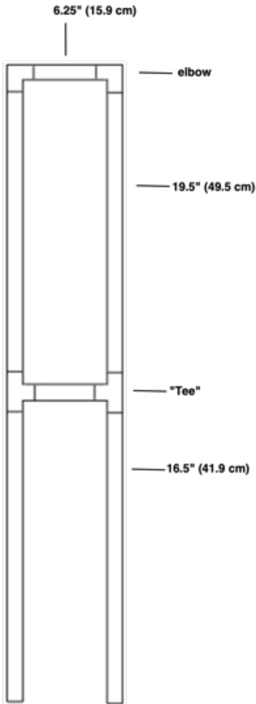
Copper Frame
